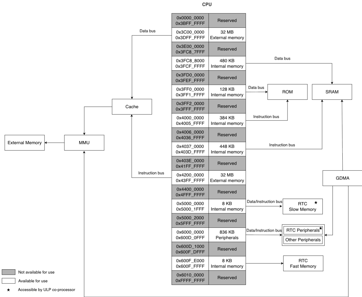
Figure 4.2-1. System Structure and Address Mapping
