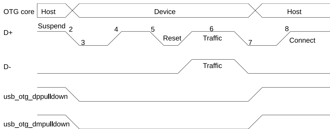
Figure 32.4-3. A-Device HNP
