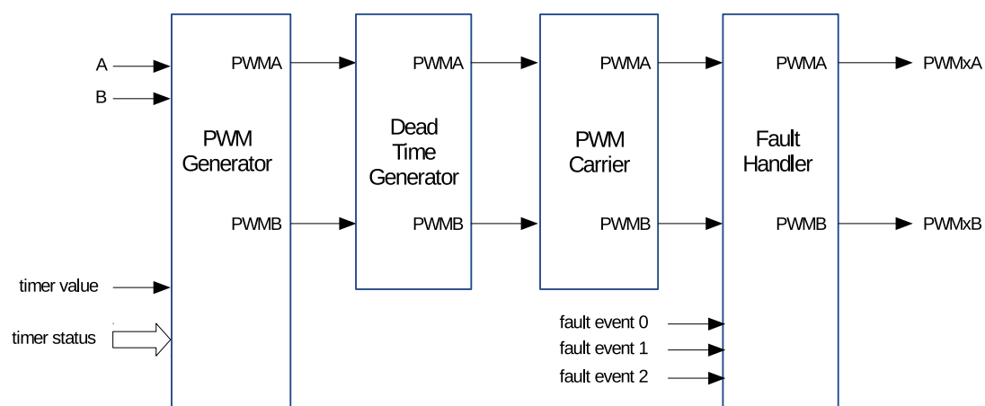
Figure 36.3-13. Submodules Inside the PWM Operator
