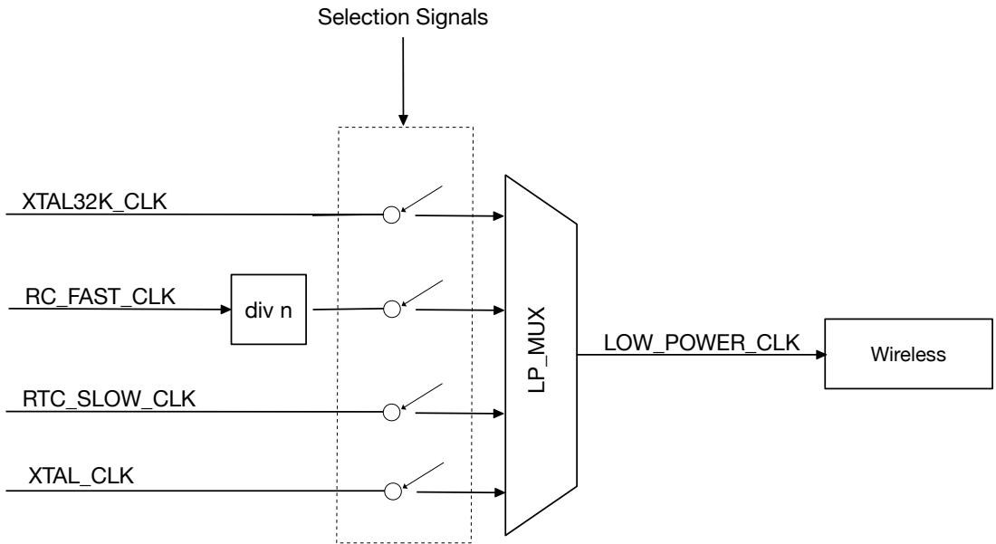
Figure 10.3-4. Wireless Clocks
