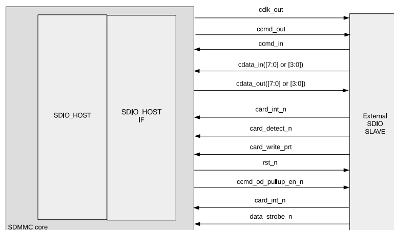
Figure 34.3-1. SD/MMC Controller External Interface Signals
