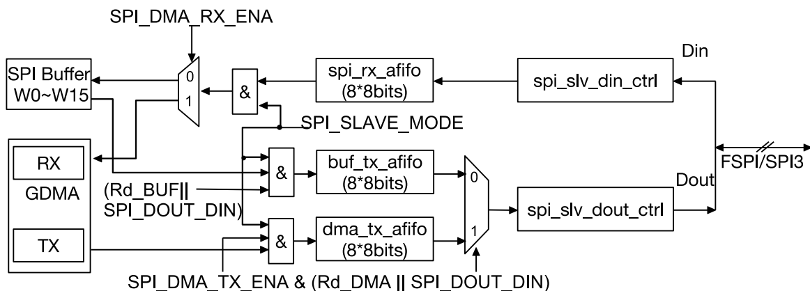
Figure 30.5-4. Data Flow Control in GP-SPI Slave Mode
