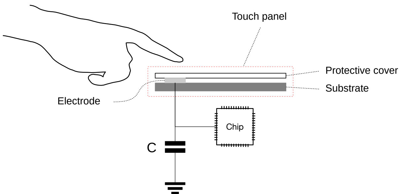
Figure 39.2-1. Touch Sensor
