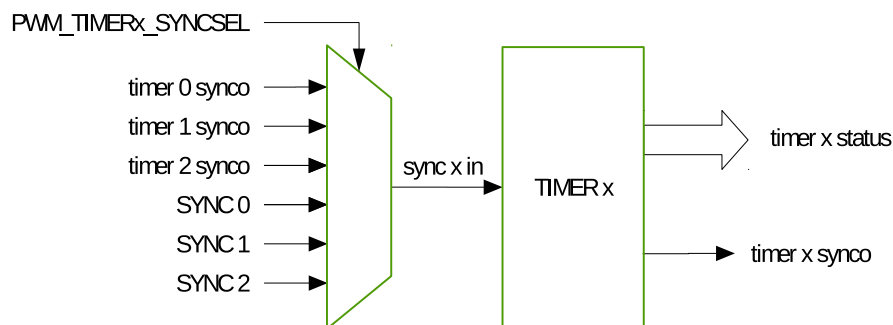
Figure 36.3-2. Timer Submodule
