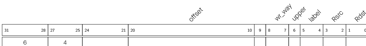
Figure 2.5-9. Instruction Type - Data Storage in Manual Storage Mode
