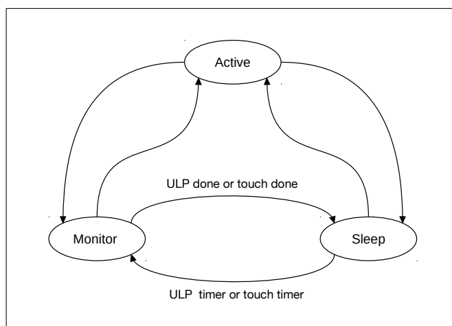
Figure 10.4-1. RTC States
