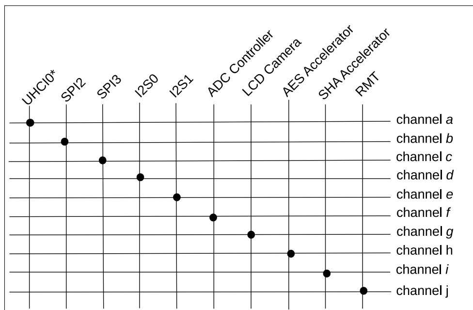
Figure 4.3-2. Peripherals/modules that can work with GDMA
