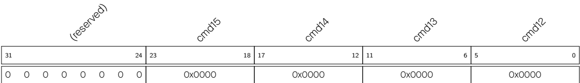
Figure 39.3-7. APB_SARADC_SAR1_PATT_TAB4_REG and Pattern Table Entry 12 - Entry 15
