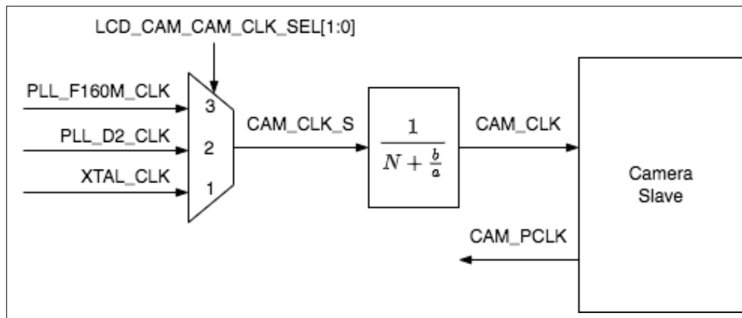
Figure 29.3-3. Camera Clock
